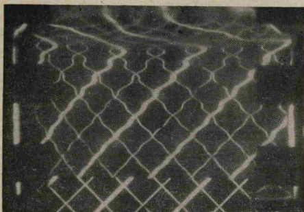
FIG. 4. Frame illustrating elastic bending wave pattern set up in stainless-steel plate when the detonation velocity is less than about 2.0 mm/ \mu sec.
